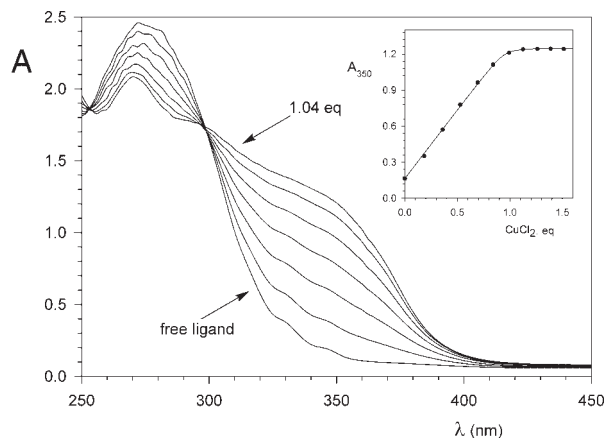
Figure 1. Variations of the UV-visible spectrum of 0.080 mM 1 on addition of increasing amounts of CuCl 2 in CH 3 OH at 25 °C. A titration plot at 350 nm is shown in the inset
