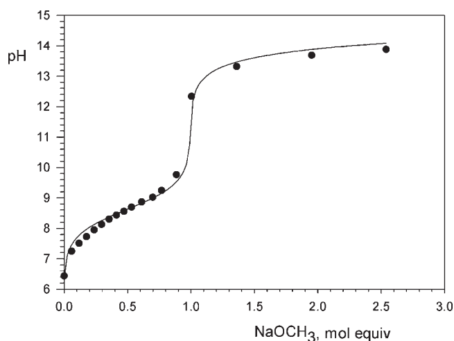
Figure 2. Potentiometric titration of a 1.30 mM 1:1 mixture of 1 and CuCl 2 in CH 3 OH at 25 °C
